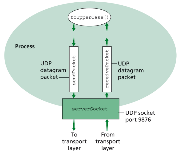
Figure 2.32 ♦ UDPSever has no streams; the socket accepts packets from the process and delivers packets to the process.
