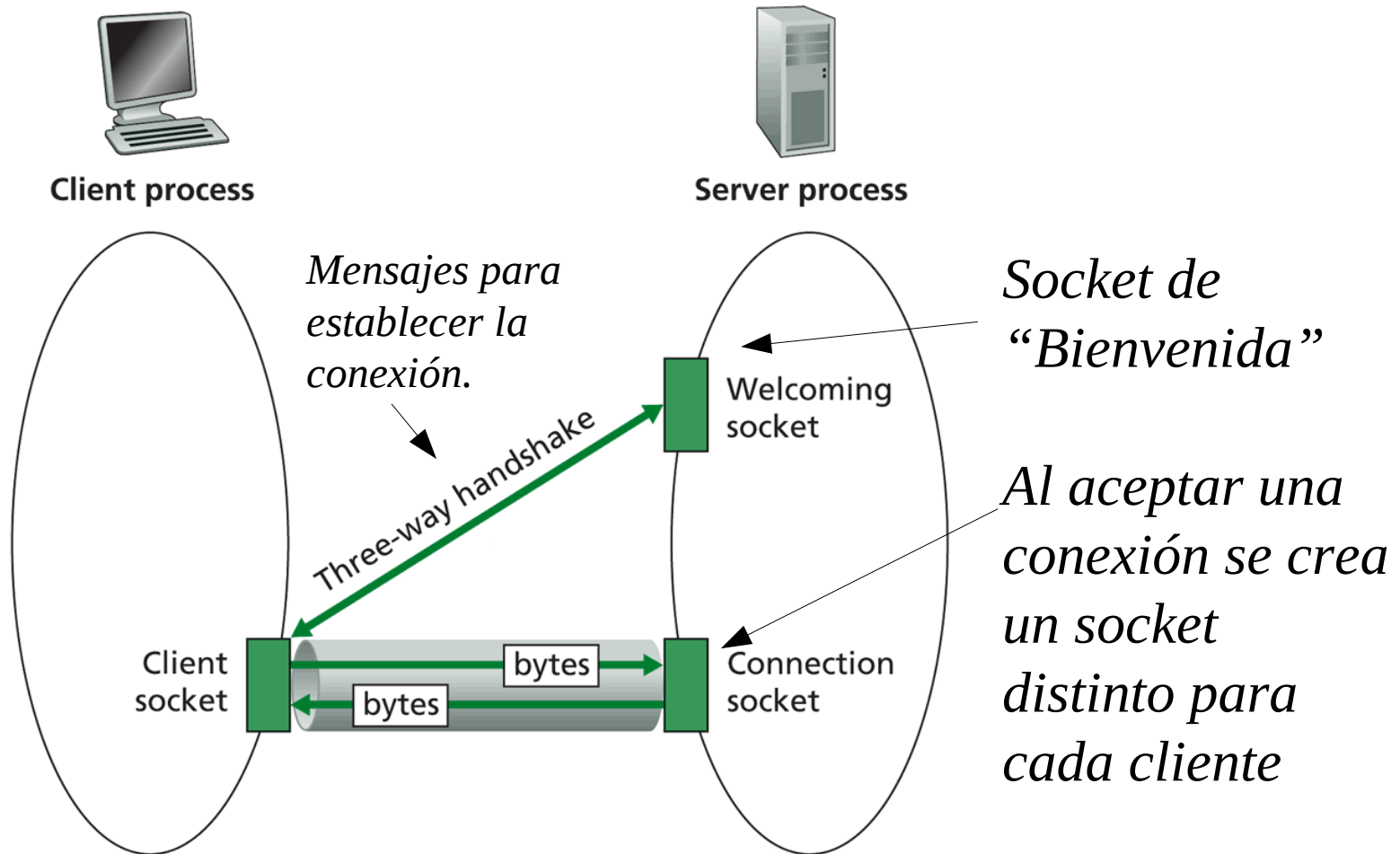
Figure 2.27 ♦ Client socket, welcoming socket, and connection socket, aplicación
